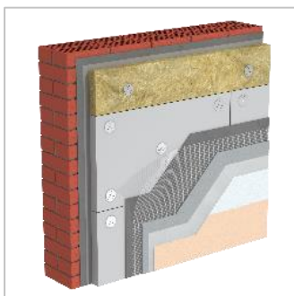
Fastening XPS on facade to decking
