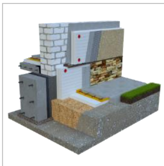
Fastening XPS to waterproofing
